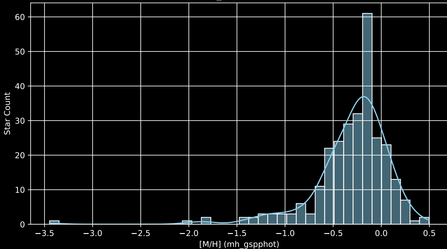
APOGEE DR17 Field: [M12-N [M/H] (mh_gspphot) (n= 279)
