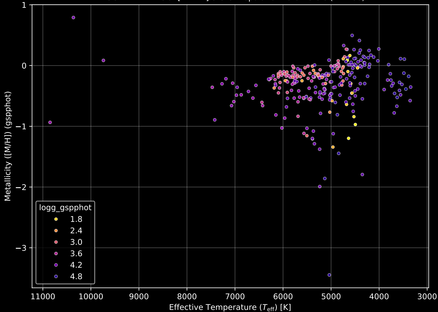
APOGEE DR17 Field: [M12-N] Stellar Population Parameters (n= 280)
