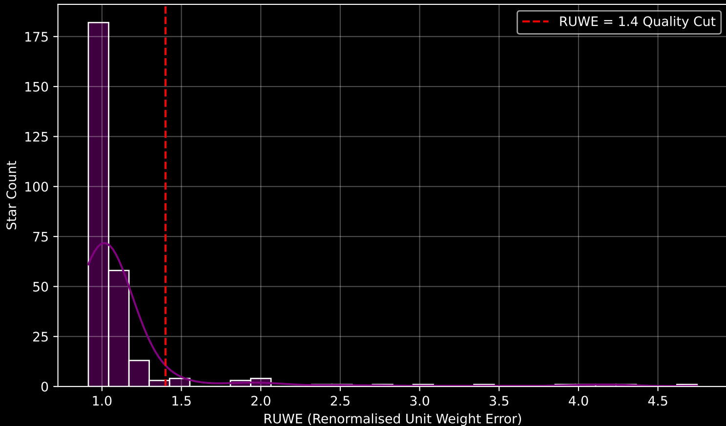
GAPOGEE DR17 Field [M12-N] RUWE Distribution (n= 277)
