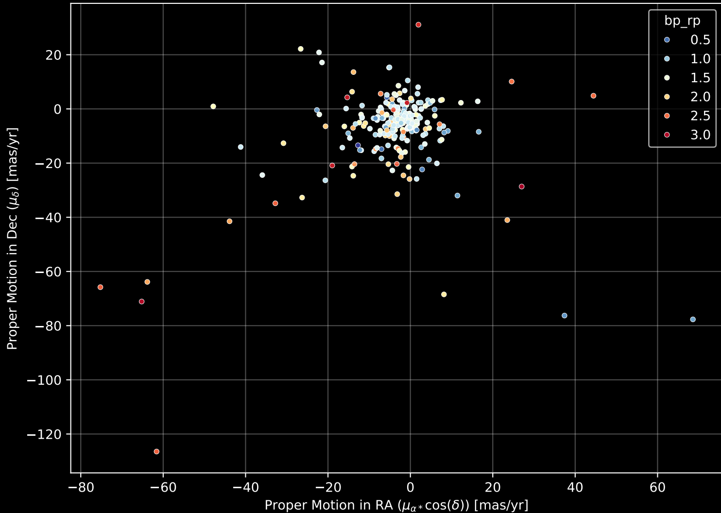
APOGEE DR17 Field: [M12-N] Proper Motion Diagram (n= 280)
