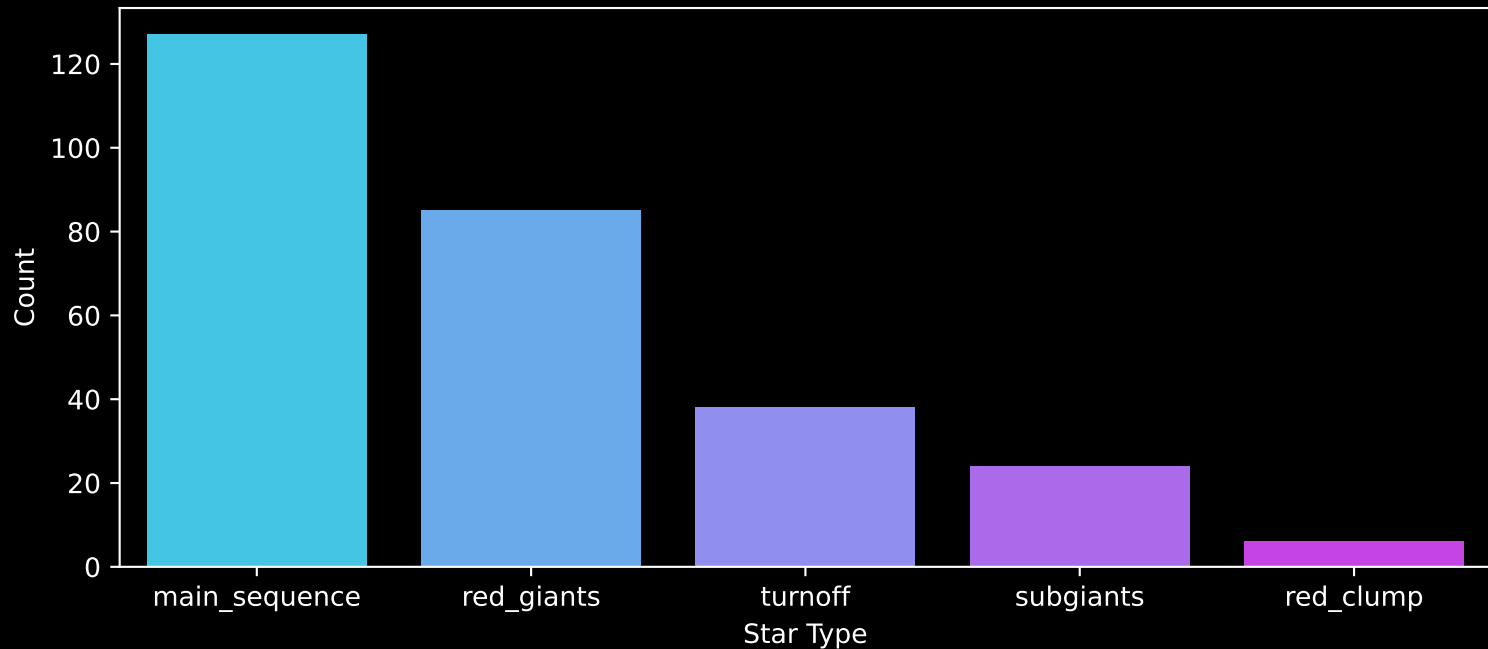
APOGEE DR17 Field: [M12-N] Count plot of Star Type
