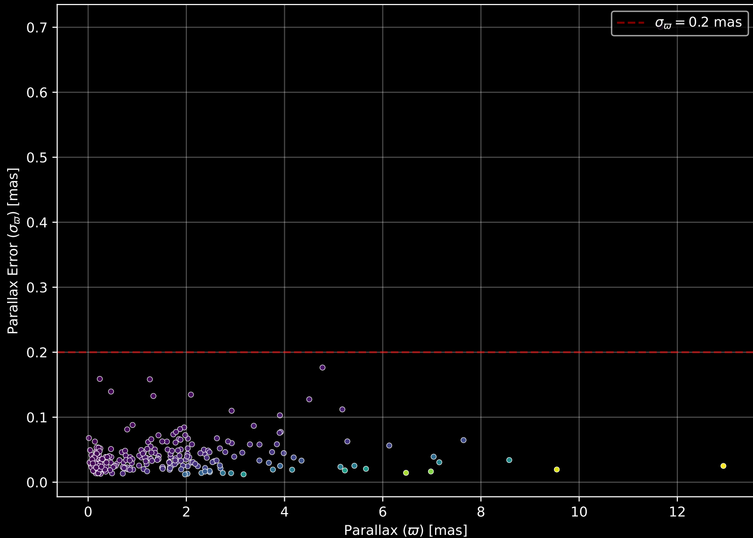
APOGEE DR17 Field: [M12-N] Parallax Quality (n= 280)
